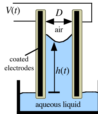
Fig. 1. Modified Pellat apparatus for aqueous liquids has vertical, parallel electrodes coated with a thin dielectric layer.
