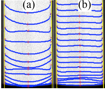
Fig. 2. Sequences of meniscus profiles at 1 ms intervals from videos. The electrode spacing D = 0.5 mm, voltage = 150 V-rms, frame rate = 1000 fps. (a) 100 Hz. (b) 100 kHz.
