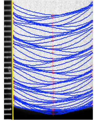
Fig. 3. Sequence of superimposed meniscus profiles captured at 1 ms intervals. Electrode spacing D = 2 mm; voltage is 150 V-rms at frequency f = 100 Hz.
