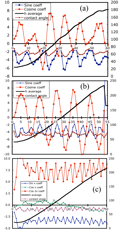
Fig. 4. Fourier components extracted from meniscus data obtained from video sequences. Spacing: D = 2 mm; voltage: V = 150 V-rms; liquid: DI water. Black curves are provided to show simultaneous time course of the rising meniscus. (a) f = 50 Hz. (b) f = 100 Hz. (c) f = 200 Hz.
