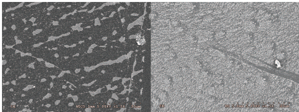
Fig. 3. MEB images ( 65.4\mu\text{m} \times 87.3\mu\text{m} ) of particles depositions at high velocities. In both case, no stick-slip occurs. They were obtain with contact-line velocities of 60\mu\text{m/s} (left) an 15\mu\text{m/s} (right), with a 3% solution.
