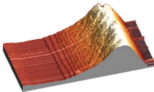
Fig. 5. AFM image of a typical particle deposition at a pinning point, obtained with a contact line velocity of 1\mu\text{m/s} (from the left to the right). The height of the defect is 1.45\mu\text{m} at the top. The lateral dimensions are 100\mu\text{m} \times 50\mu\text{m} . The parallel lines that can be seen at the bottom of the defect corresponds to successive stairs of particles layers.
