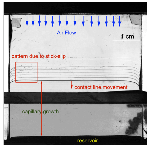
Fig. 1. Optical image of the capillary growth during a typical experiment. The cell thickness is 0.45 mm. On this image, horizontal patterns can be seen above the capillary growth. Contact line velocity is 500 nm/s, particle volume fraction is 3%.
